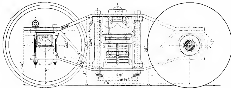
Fig. 4748. Sectional Side Elevation.
